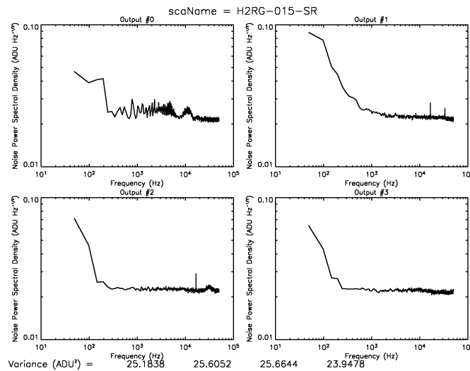
Figure 18. The Fourier Power Spectrum of the IDTL test setup for Rochwell HAWAII-2RG SCAs is mostly flat. The most obvious component is a \sim 1/f tail at low frequencies. Our measurements indicate that the test setup contributes about 8 e - rms per correlated double sample in this configuration. This corresponds to about 3 e - rms per Fowler-8 exposure which is well below the JWST 9 e - requirement for the detector.
