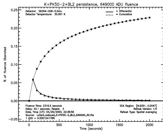
Figure 34: Three-reset persistence for Rockwell H2RG-015-5.0mu (top row) and Raytheon SB304-008-5.0mu (bottom row). Results are for the K+PK50-2+BL2 filter combination. The notation “BL2” refers to a combination of two 1% Inconel neutral density filters, while “PK50-2” refers to a 2-mm thick PK50 filter.
