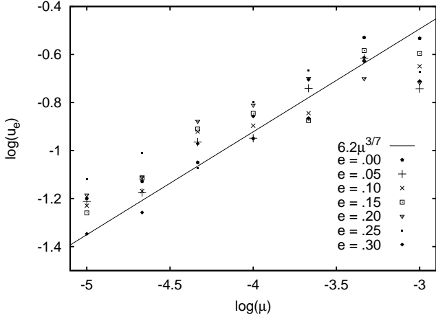
Figure 2. Eccentricity dispersion, u_e , in the disk edge as a function of planet mass. The line shown is u_e = 6.2\mu^{3/7} and consistent with that predicted with equation 17 for particles near a planet in a circular orbit. Each point type corresponds to integrations containing a planet with a different eccentricity. The eccentricity dispersion is not strongly dependent on the planet eccentricity.
