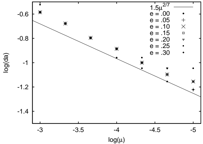
Figure 1. The distance between the planet semi-major axis and that of the chaotic zone boundary is plotted as a function of planet mass ratio, \mu . Points are plotted at the semi-major axis at which particles lifetime exceeded 10^4 orbits. Each point type corresponds to different planet eccentricity. The points lie on top of one another because the chaotic zone width is independent of the planet eccentricity for orbits with zero free eccentricity. Particles were initially placed in orbits with zero free eccentricity and arguments of peri-astron the same as the planet. The solid line corresponds to that predicted by equation 1.
