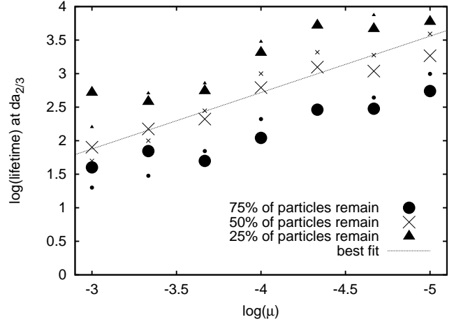
Figure 3. Particle lifetime in planetary orbits as a function of planet mass for particles with initial semi-major axis 2/3 of the way between the planet’s semi-major axis and the chaotic zone boundary. Large and small points are for planet eccentricity e_p = 0.05 and 0.2 , respectively. The circles, crosses and triangles correspond to times when 75%, 50% and 25% of the particles remain in the simulation, respectively. The line shown has lifetime equal to 0.23\mu^{-0.84} . Particles have initial angle of pericenter identical to that of the planet and zero free eccentricity. The lifetimes are not strongly dependent on the planet eccentricity.
